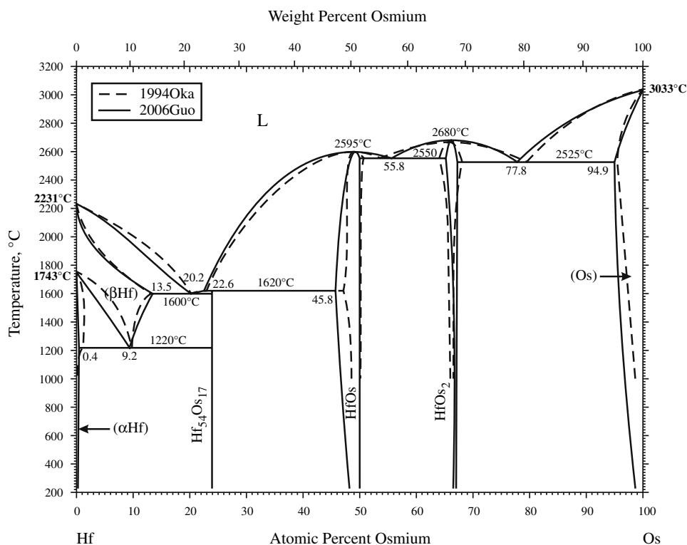
Fig. 1 Hf-Os phase diagram
